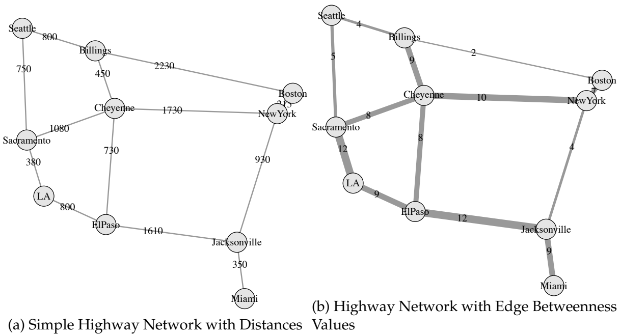
Figure 3: Illustrating Edge Betweenness
